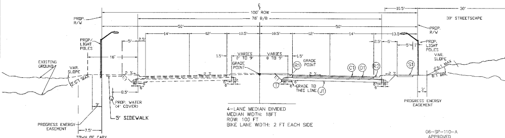
O'KELLY CHAPEL ROAD STATION 20+69.53 TO 21+50
