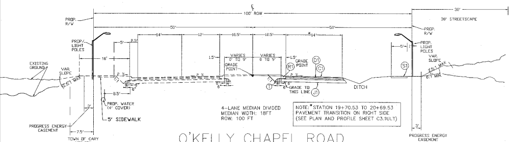
O'KELLY CHAPEL ROAD STATION 13+25 TO 20+69.53
