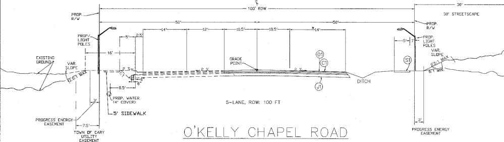
O'KELLY CHAPEL ROAD STATION 10+40 TO 11+70
