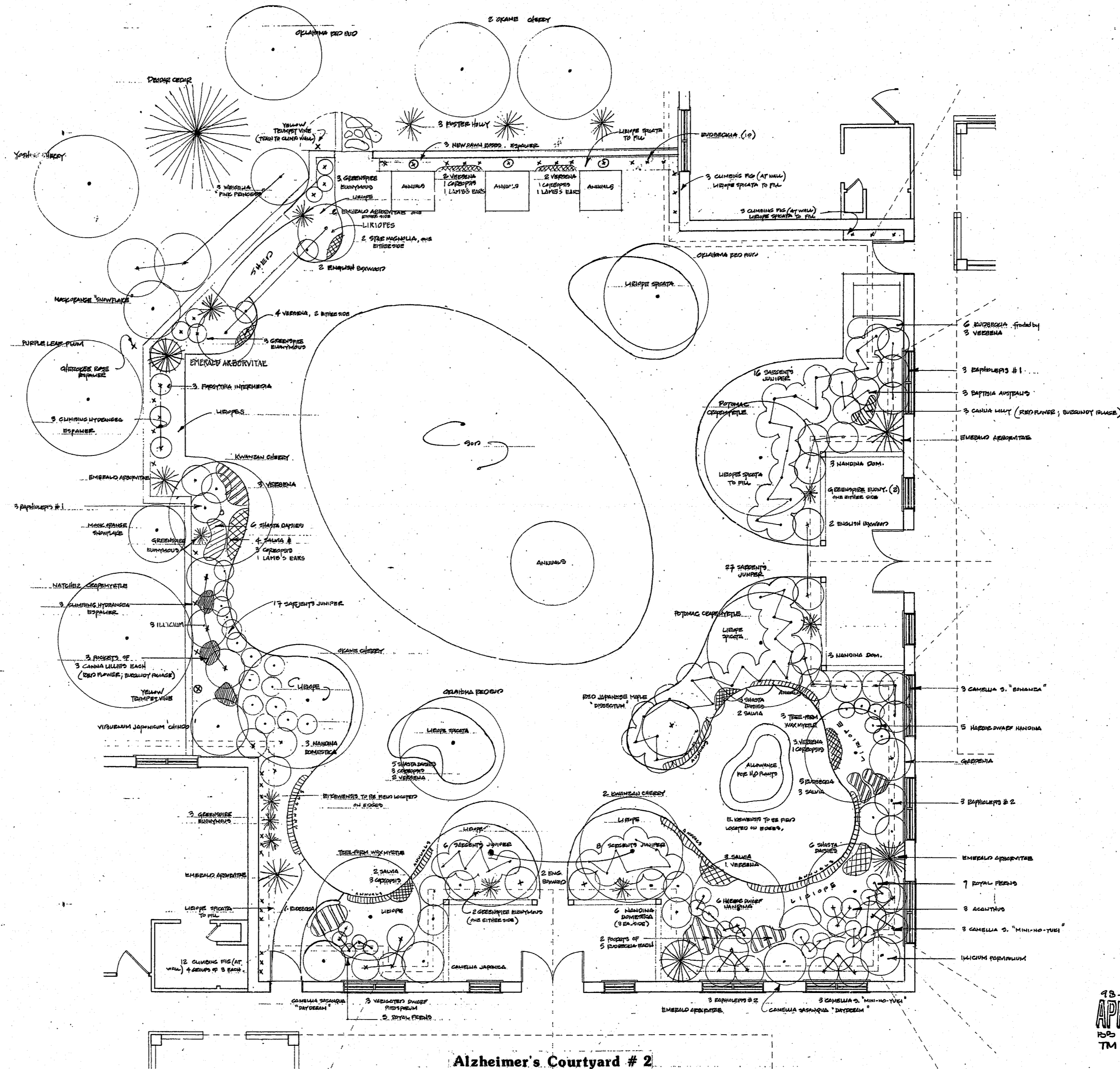
Alzheimer's Courtyard # 2 ALL DEPS TO BE 20/60 TOPSOIL MIX FROM BRADSHAW CONTRACTING OR EQ.
