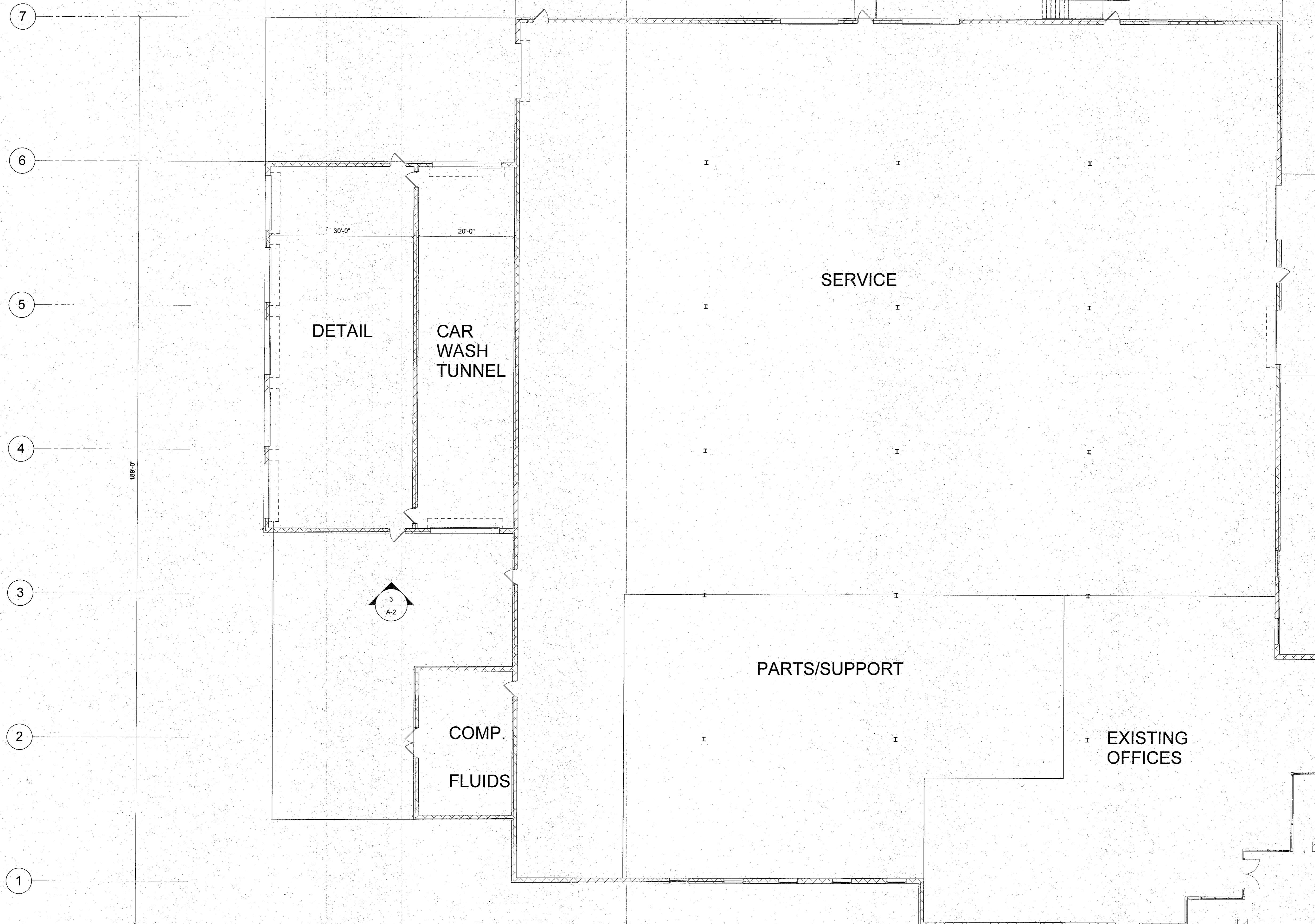
FLOOR PLAN 1 A-1 3/32" = 1'-0"
