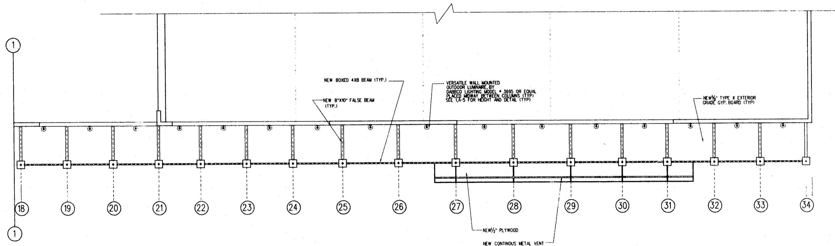
2 PARTIAL REFLECTED CEILING PLAN A-9 Not To Scale
