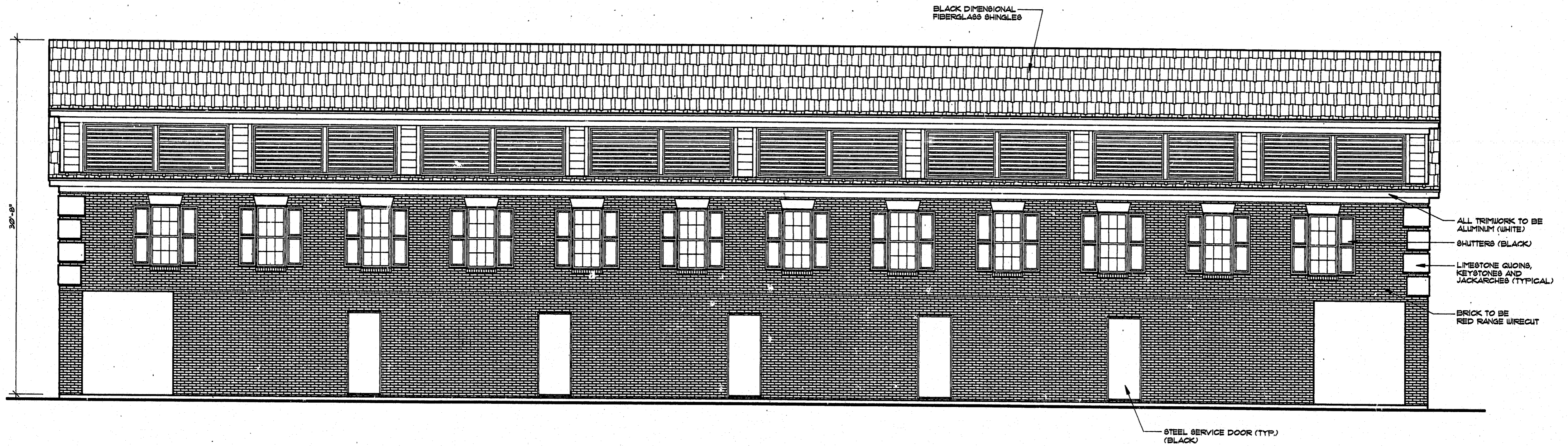
REAR ELEVATION
