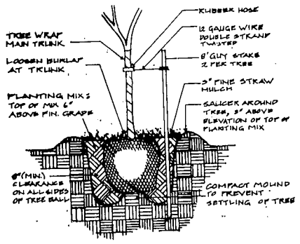
0-3" CALIPER TREE NOT TO SCALE
