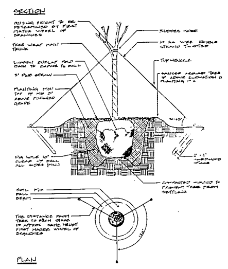
LARGE TREE PLANTING NOT TO SCALE
