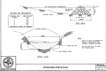
STANDARD CHECK DAM
