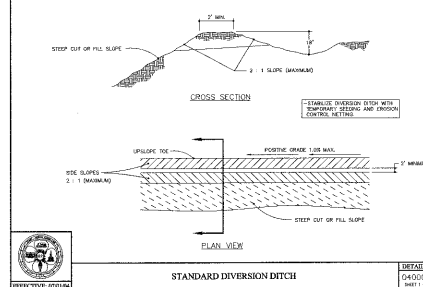
STANDARD DIVERSION DITCH
