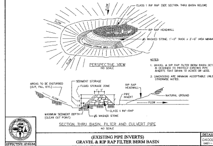
GRAVEL & RIP RAP FILTER BASIN (EXISTING PIPE INVERTS)
