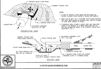
CATCH BASIN RISER/FILTER
