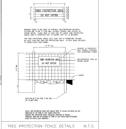
TREE PROTECTION FENCE DETAILS N.T.S.
