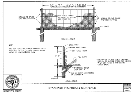
STANDARD TEMPORARY SILT FENCE
