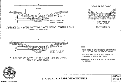
STANDARD RIP-RAP LINED CHANNELS
