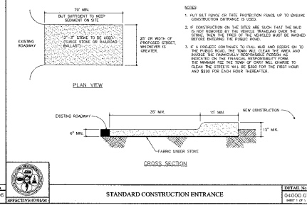
STANDARD CONSTRUCTION ENTRANCE
