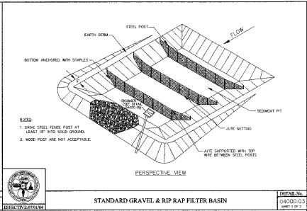
STANDARD GRAVEL & RIP RAP FILTER BASIN
