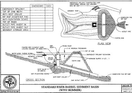
STANDARD RISER-BARREL SEDIMENT BASIN (WITH SKIMMER)
