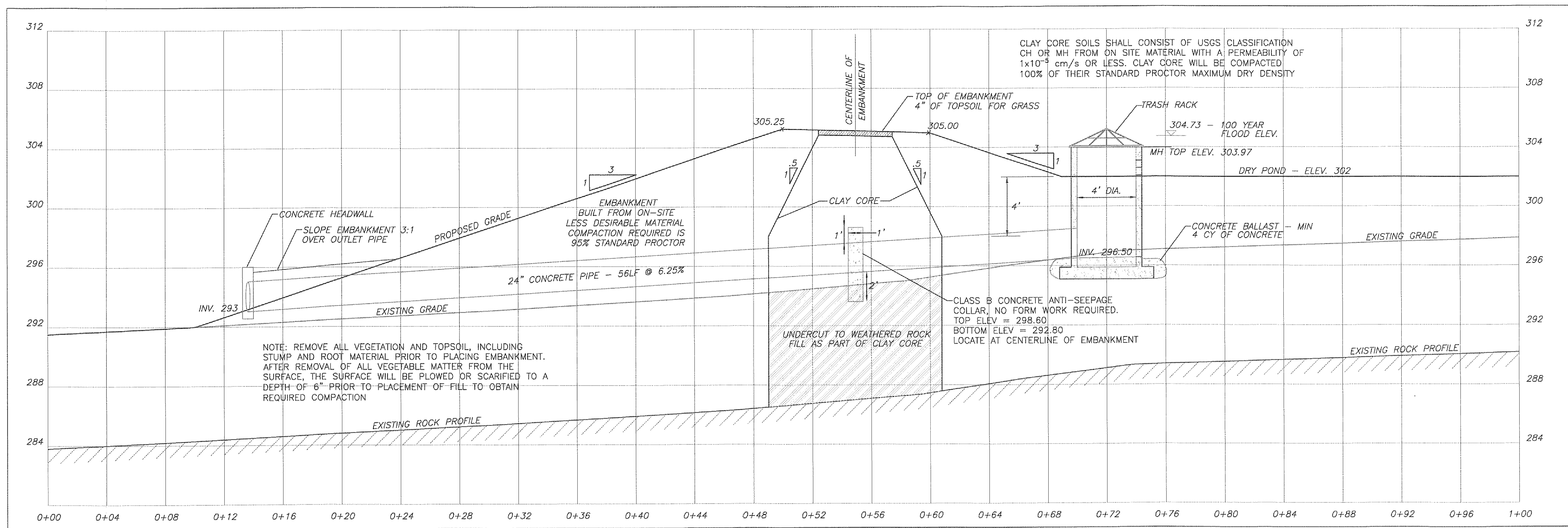
1 DRY POND DAM DETAIL C805 SCALE 1"=4'
