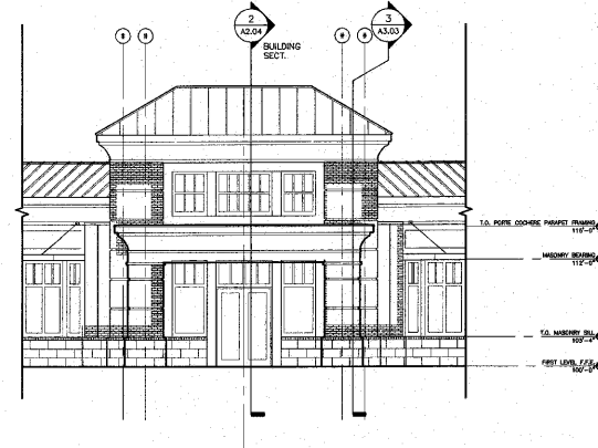
03 ENTRY ELEVATION (PLAN SOUTHWEST)
