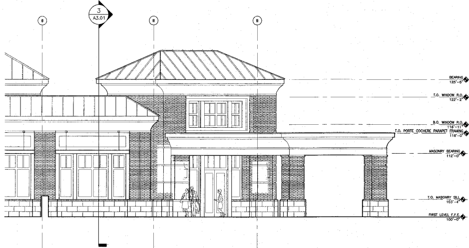
04 ENTRY ELEVATION (PLAN WEST)
