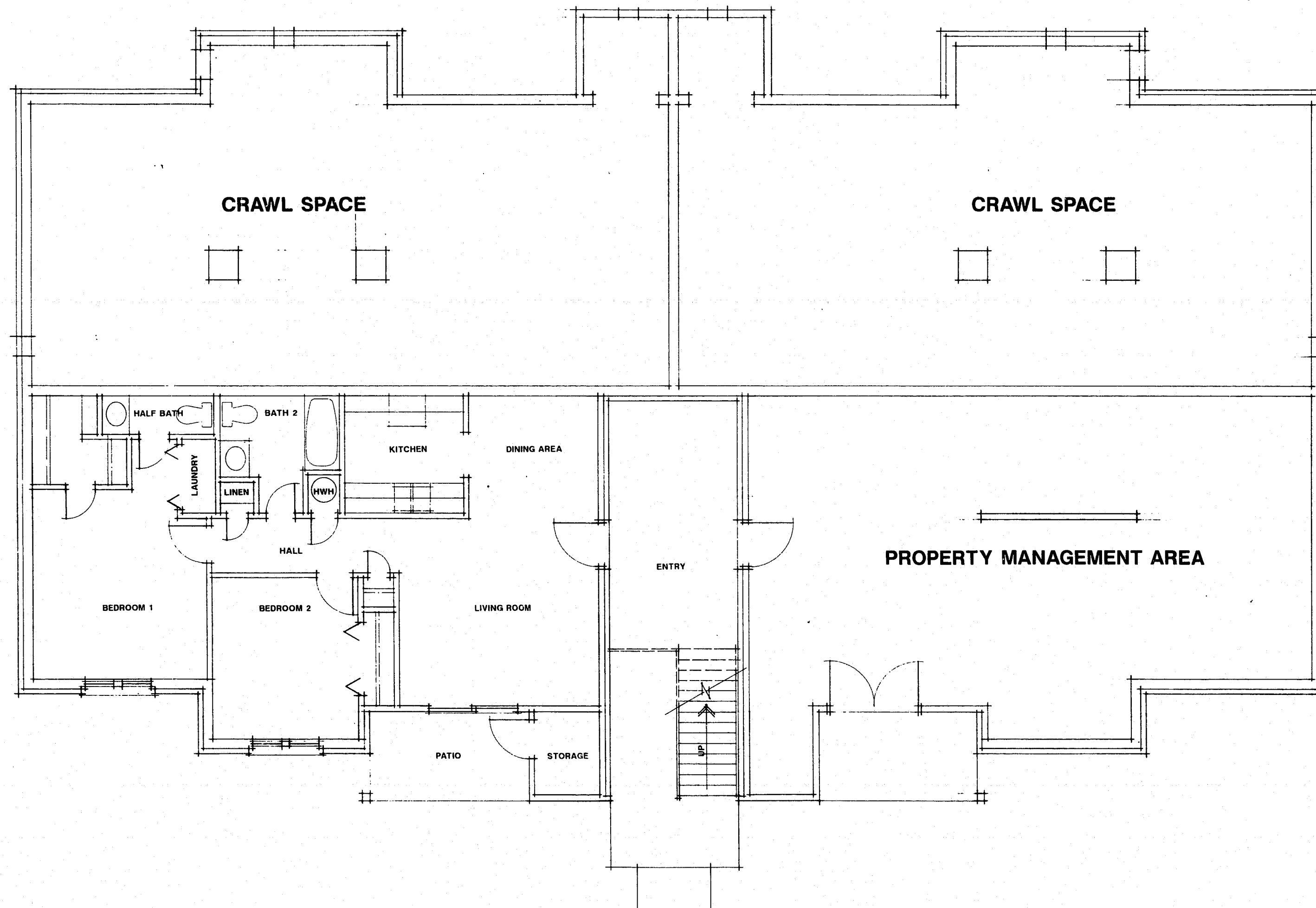
LOWER LEVEL FLOOR PLAN SCALE: 1/4" = 1'-0"
