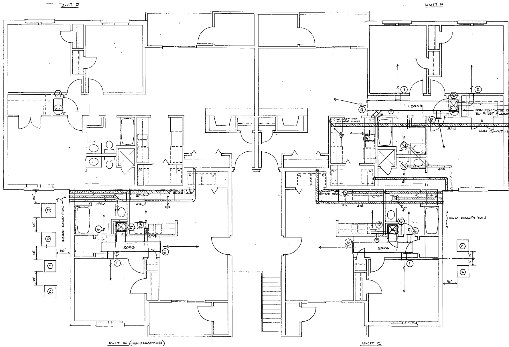
1 1/2 BED ROOM FLOOR PLAN-MECHANICAL 1/4" = 1'-0"
