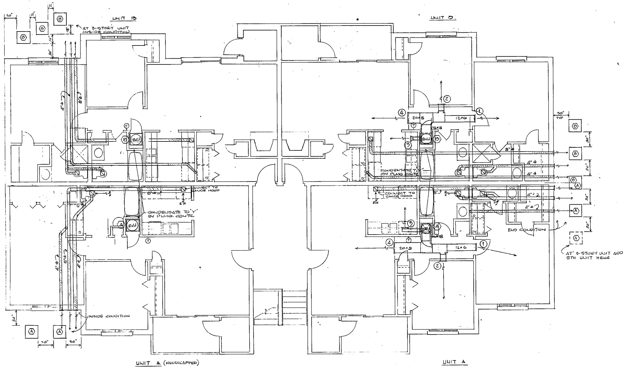
2 BED ROOM FLOOR PLAN - MECHANICAL 1/4" = 1'-0"
