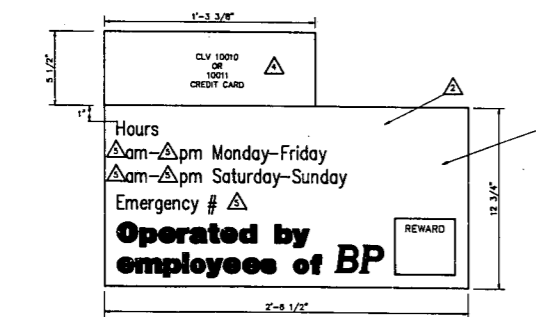
4 DETAIL - TYPICAL LAYOUT SCHEME B
