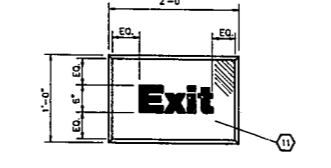
15 DETAIL - GRAPHICS
