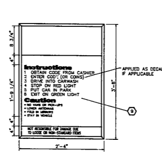
14 DETAIL - CAR WASH/INFORMATION SIGN
