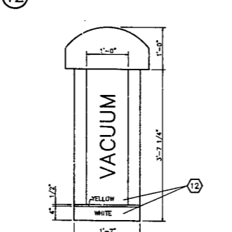
13 DETAIL - VACUUM
