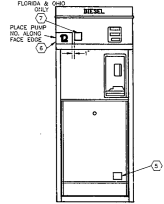
DECAL PLACEMENT WAYNE DIESEL MODEL DL1/367-IL/19G
