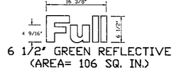
6 1/2" GREEN REFLECTIVE (AREA= 106 SQ. IN.)
