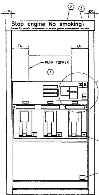
DECAL PLACEMENT GILBARCO MPD-3
