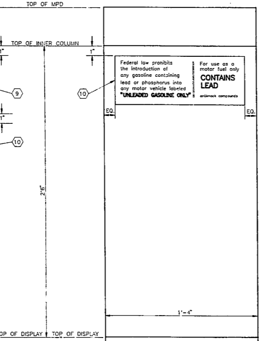
INNER COLUMN MPD DECAL PLACEMENT OR & WA
