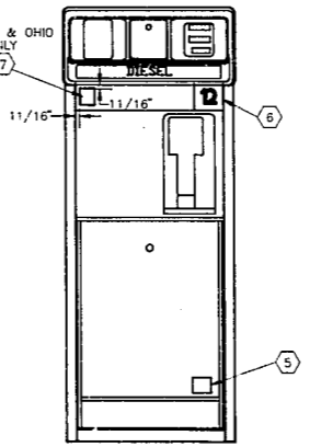
DECAL PLACEMENT GILBARCO DIESEL MODEL 5921-S2 DUAL SALESMAN II
