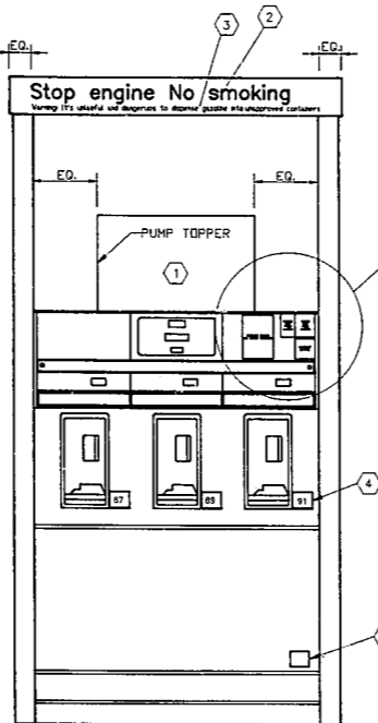
DECAL PLACEMENT WAYNE MGD
