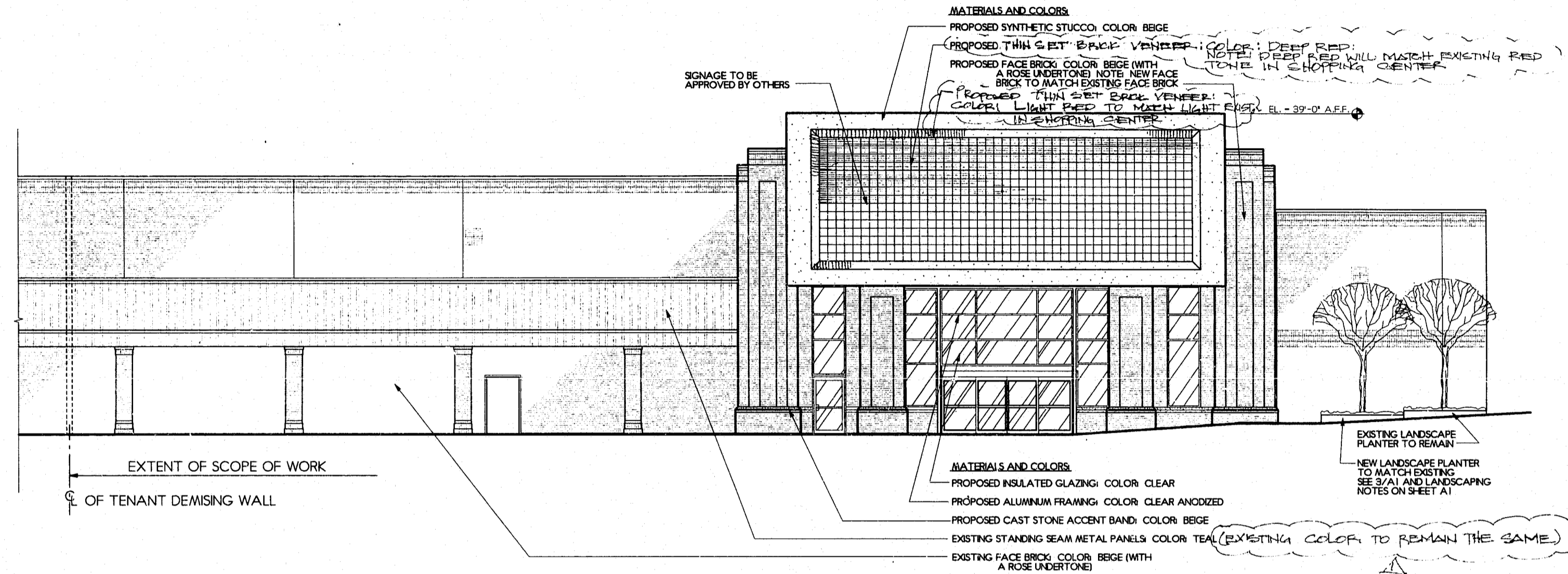
1 FRONT ELEVATION A2 1/8" = 1'-0"
