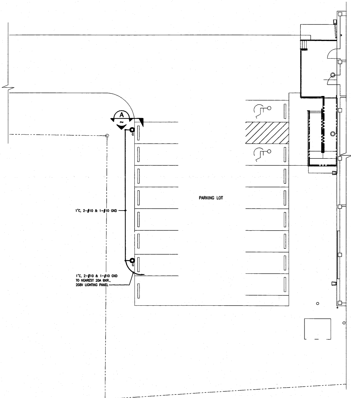
OUTDOOR LIGHTING PLAN
