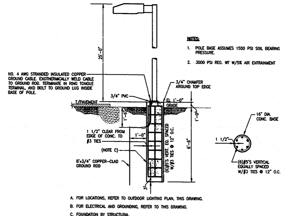
LIGHT POLE BASE DETAIL
