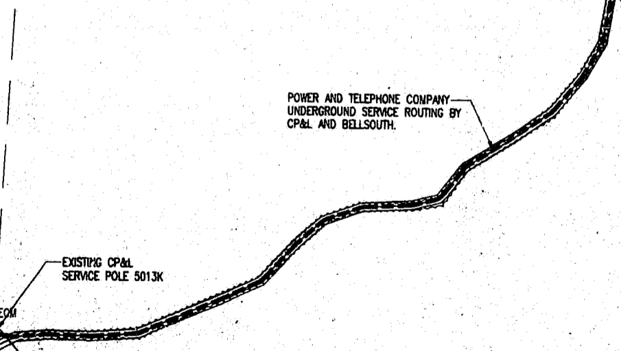
SERVICES ROUTING PLAN SCALE: 1" = 100'
