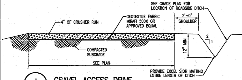
3 GRAVEL ACCESS DRIVE C5 C7 SCALE: NONE
