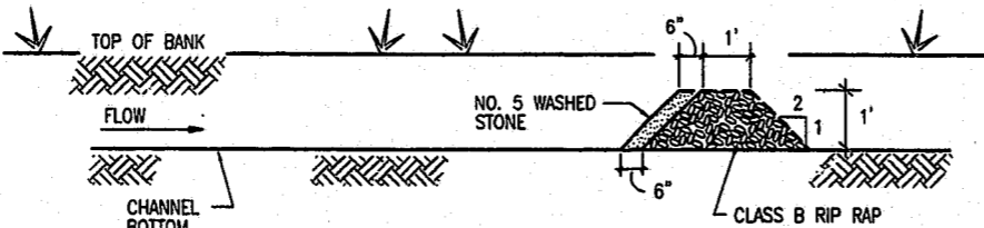
1 STONE CHECK DAM C5 C8 SCALE: NONE
