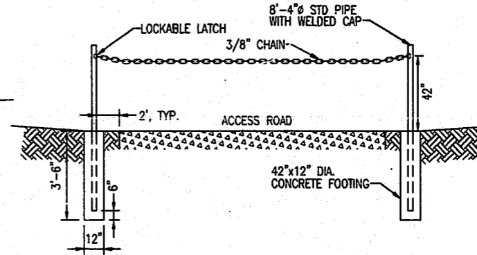
4 CHAIN GATE DETAIL C5 C7 SCALE: NONE
