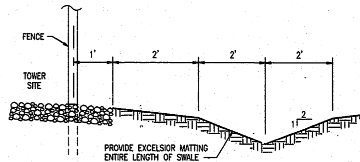
2 GRASS LINED SWALE C5.2 C8 SCALE: NONE
