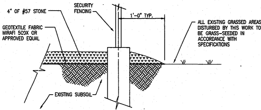
1 GRAVEL EDGE AT FENCE DETAIL C5 C7 SCALE: NONE
