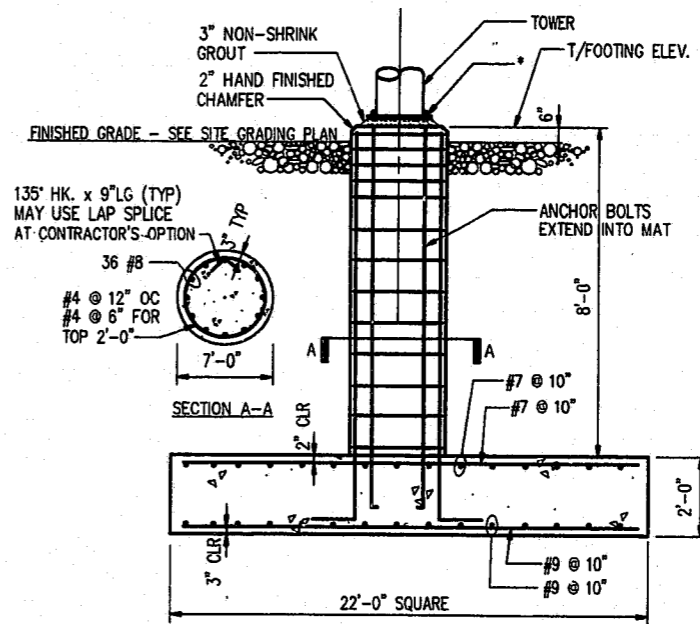
SECTION @ MONOPOLE FOUNDATION NO SCALE
