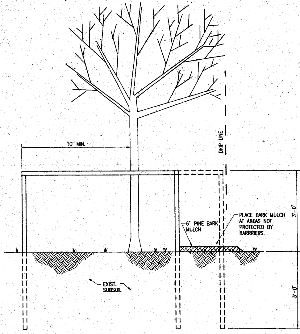
1 TREE PROTECTION BARRICADE SCALE: NONE
