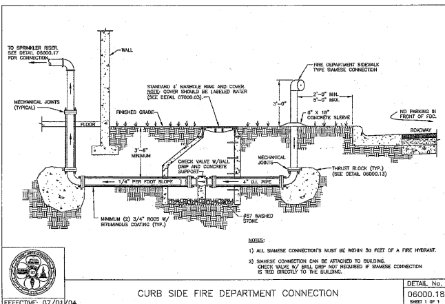
CURB SIDE FIRE DEPARTMENT CONNECTION
