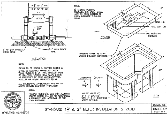
STANDARD 1 1/2" & 2" METER INSTALLATION & VAULT
