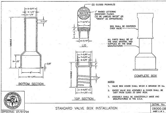
STANDARD VALVE BOX INSTALLATION
