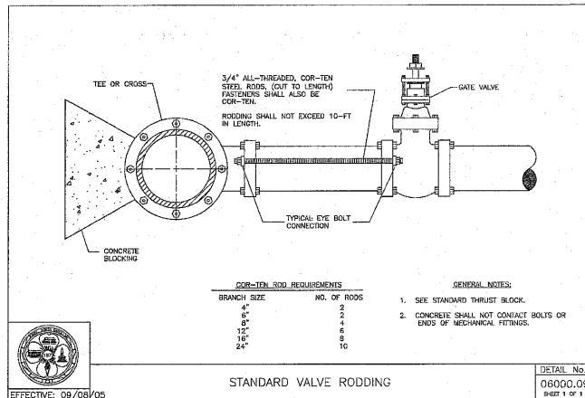
STANDARD VALVE RODGING
