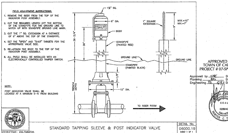
STANDARD TAPPING SLEEVE & POST INDICATOR VALVE
