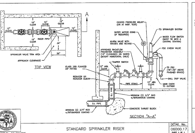
STANDARD SPRINKLER RISER
