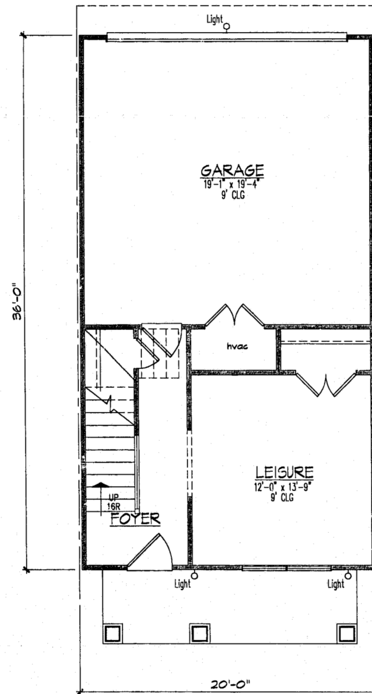
LOWER LEVEL 1/4" = 1'-0"
