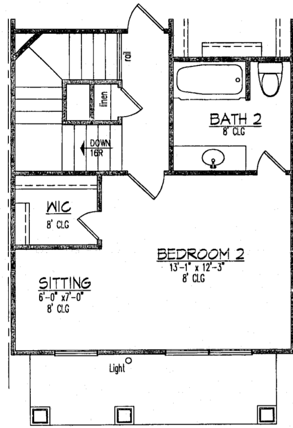
OPTIONAL BEDROOM 2 w/SITTING & PRIVATE BATH 1/4" = 1'-0"
