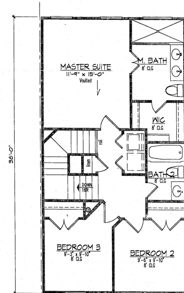
THIRD FLOOR PLAN 1/4" = 1'-0"
