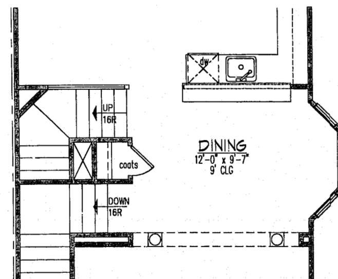
OPTIONAL BAY WINDOW @ DINING (END UNIT ONLY) 1/4" = 1'-0"
