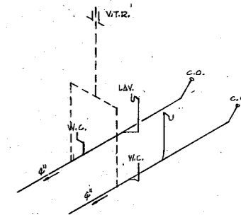
WASTE RISER NO. 2
