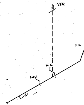
WASTE RISER NO. 1
