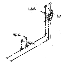
WATER RISER NO. 2
