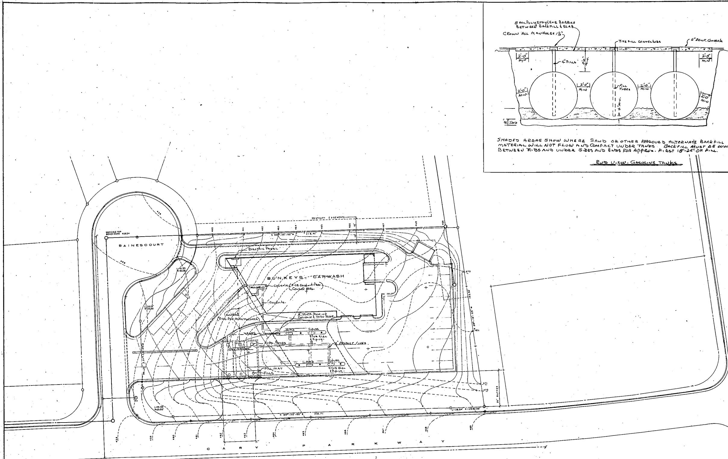
⊕ SITE PLAN - GASOLINE SCALE 1" = 20'-0"
