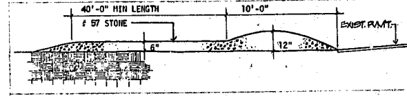
SECTION 'N' TEMPORARY CONSTRUCTION ACCESS NO SCALE
