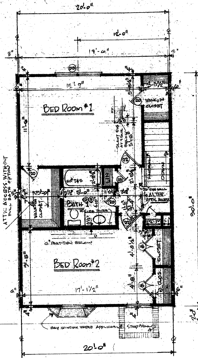
UPPER LEVEL FLOOR PLAN (2BR)
