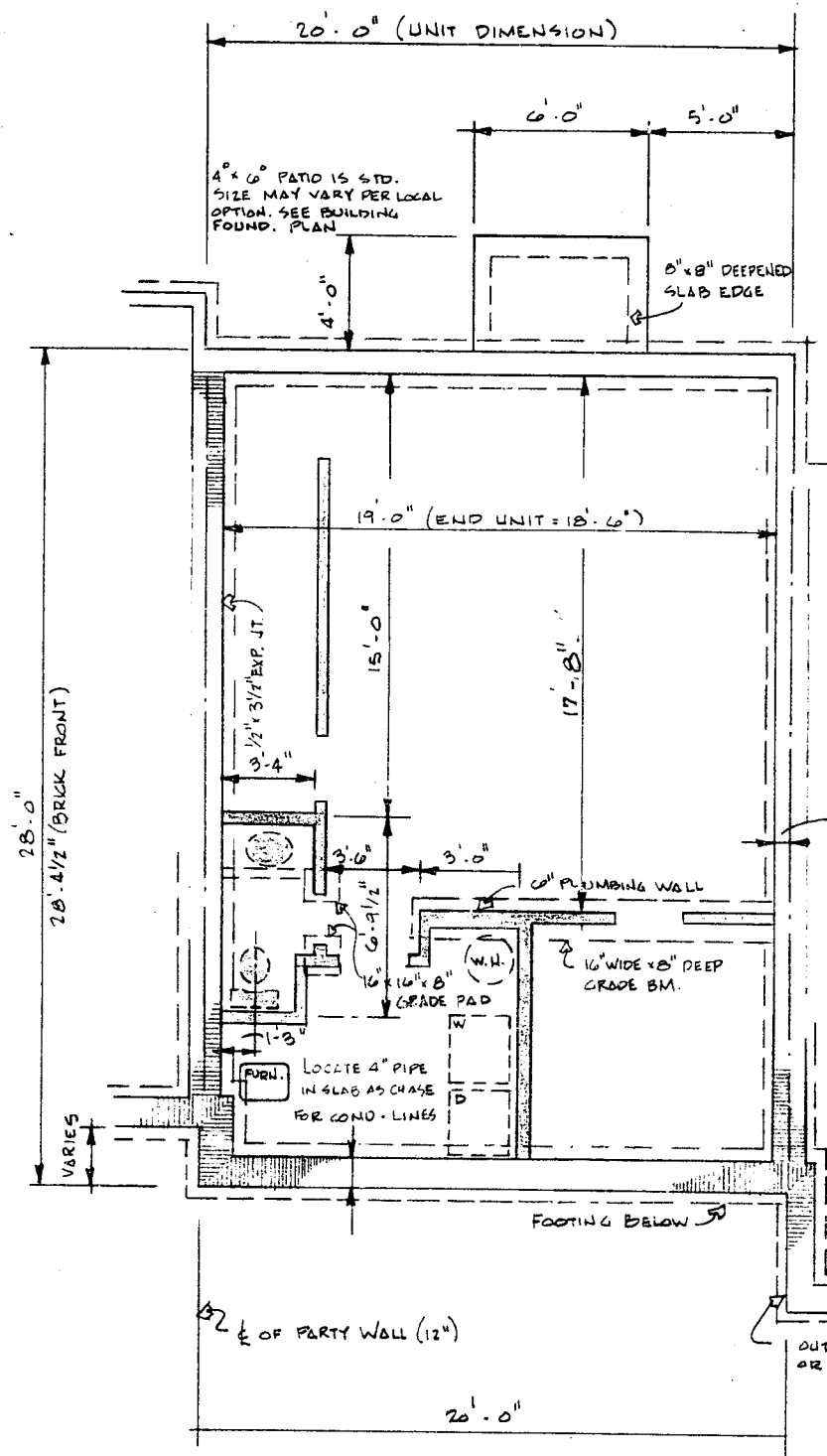
FOUNDATION PLAN
