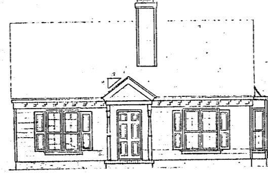
KH-5128 RD-R (SLAB)
