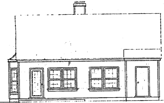
TYPICAL KH-5120 RD-R REAR ELEVATION
