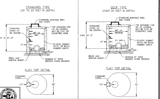
STANDARD PRECAST CONCRETE MANHOLE JUNCTION BOX DETAIL NO. 08000.05 SHEET 1 OF 2
