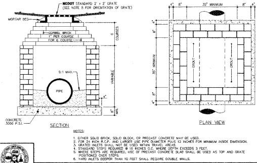
STANDARD YARD INLET WITH GRATE AND FRAME DETAIL NO. 08000.02 SHEET 1 OF 2
