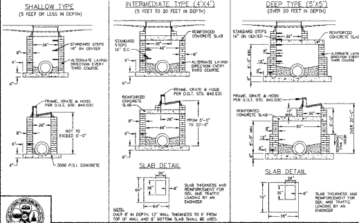
STANDARD CONCRETE BLOCK OR BRICK CATCH BASIN DETAIL NO. 08000.03 SHEET 1 OF 2
