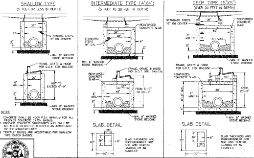
STANDARD PRECAST CONCRETE CATCH BASIN DETAIL NO. 08000.03 SHEET 1 OF 2
