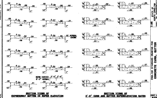
ENGLISH STANDARD DRAWINGS FOR CONCRETE CURB AND GUTTER DETAIL NO. 846.01 SHEET 1 OF 2
