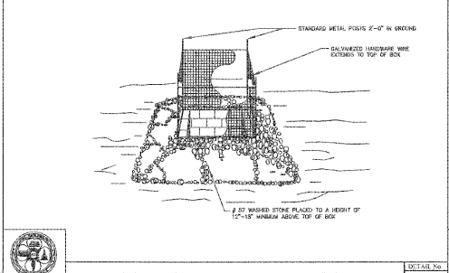
STANDARD BLOCK & GRAVEL DROP INLET PROTECTION
