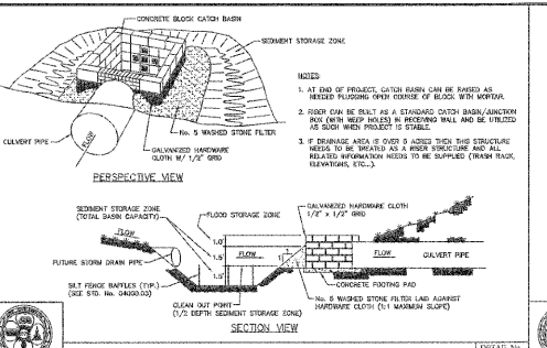
CATCH BASIN RISER/FILTER
