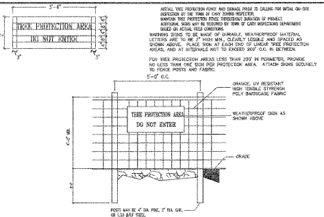
TREE PROTECTION FENCE DETAILS N.T.S.
