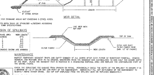
STANDARD GRAVEL & RIP-RAP FILTER BASIN
