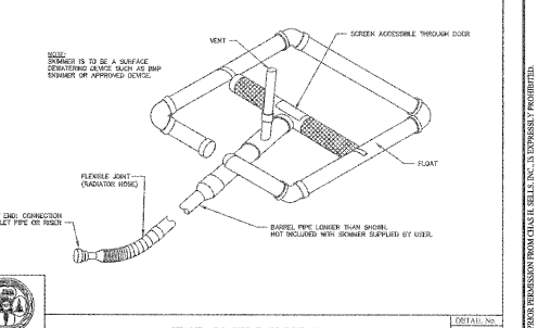
STANDARD SKIMMER DETAIL
