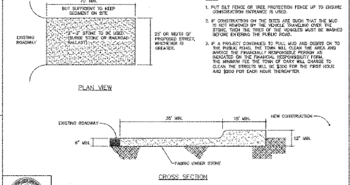
STANDARD CONSTRUCTION ENTRANCE
