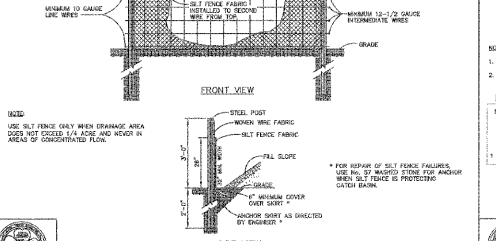
STANDARD TEMPORARY SILT FENCE
