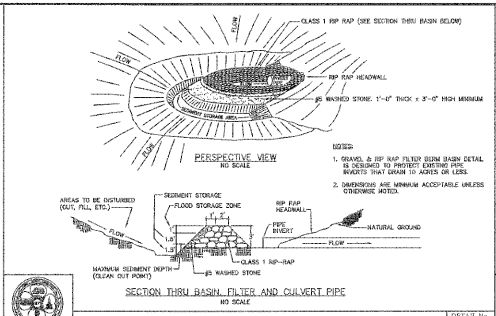
SECTION THRU BASIN FILTER AND CULVERT PIPE
