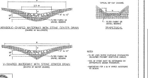
STANDARD RIP-RAP LINED CHANNELS
