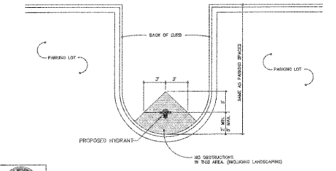
STANDARD HYDRANT LOCATION (FOR PARKING LOT)
