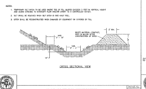
STANDARD TEMPORARY SILT DITCH
