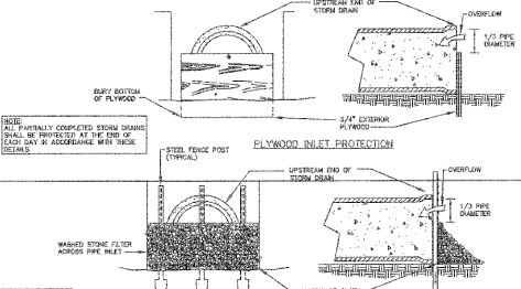
STANDARD PIPE INLET PROTECTION (PLYWOOD & STONE)
