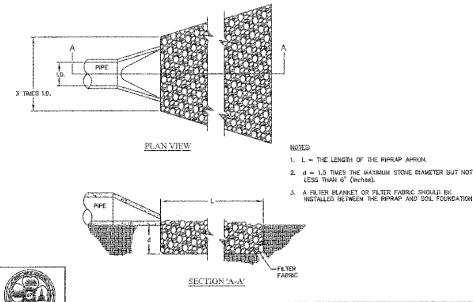
STANDARD CATCH BASIN/YARD INLET PROTECTION
