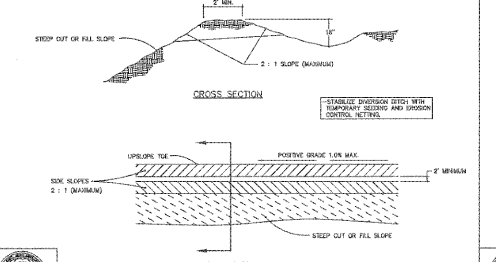
STANDARD DIVERSION DITCH
