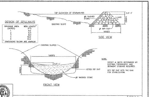
STANDARD CHECK DAM
