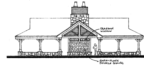
Rear Elevation
