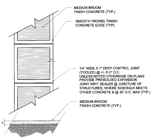
4. Concrete Sidewalk Scale: 1/2" = 1'-0"
