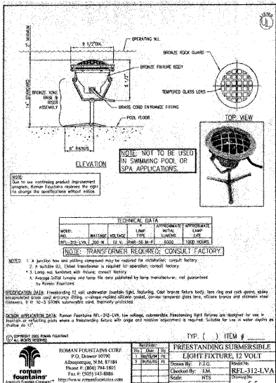
2. Underwater Uplight Not to Scale
