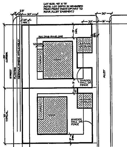
NEIGHBORHOOD HOUSE TYPE 2 ALLEY-LOADED GARAGE
