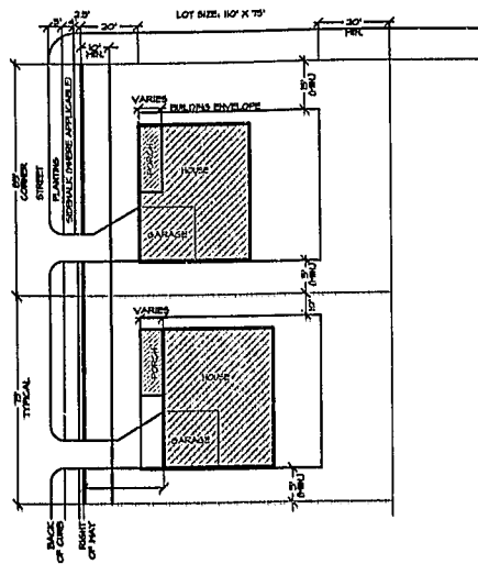
NEIGHBORHOOD HOUSE TYPE 2 FRONT LOADED GARAGE
