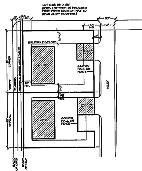
NEIGHBORHOOD HOUSE TYPE 1 ALLEY LOADED GARAGE
