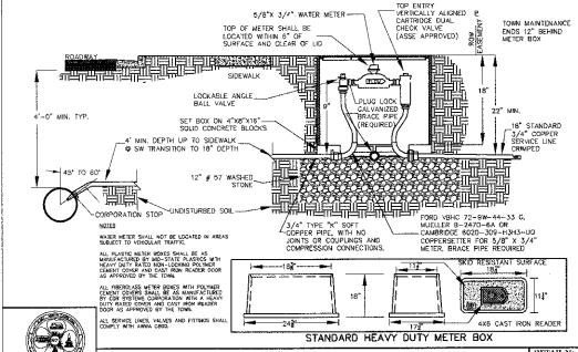
STANDARD 3/4" WATER SERVICE & METER BOX INSTALLATION DETAIL NO. 06000.01
