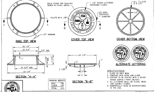
STANDARD MANHOLE RING AND COVER (TYPE I PAVED AREAS) STD. NO. 6.14
