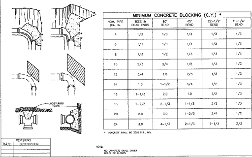
STANDARD REACTION BLOCKING STD. NO. 6.12
