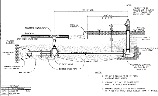
STANDARD HYDRANT INSTALLATION STD. NO. 6.06
