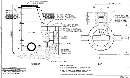
STANDARD OUTSIDE DROP MANHOLE STD. NO. 7.06
