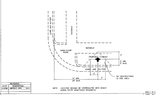
STANDARD HYDRANT LOCATION STD. NO. 6.07
