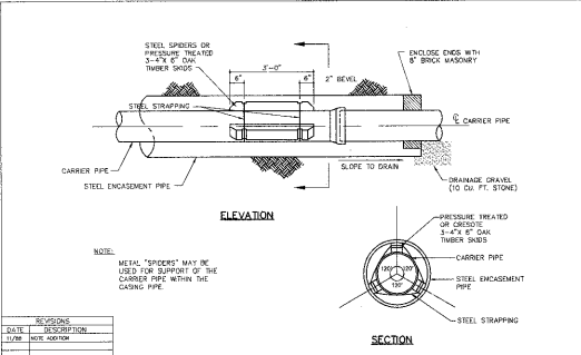
CARRIER PIPE STD. NO. 5.02
