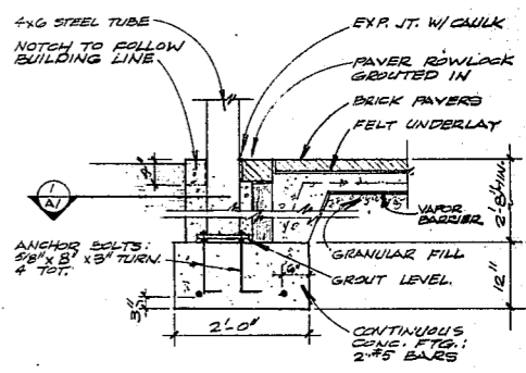
2 SECTION 3/4" = 1'-0"
