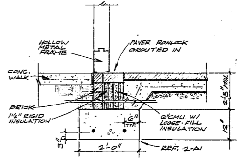
3 SECTION 3/4" = 1'-0"
