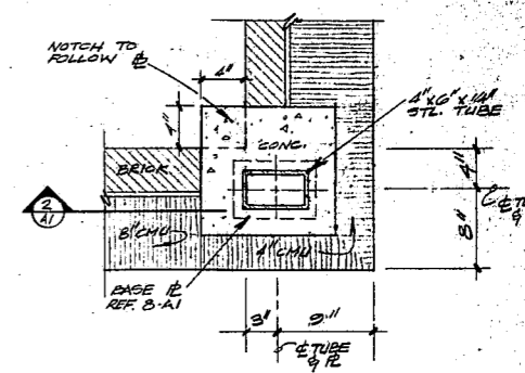
1 PLAN DETAIL 1/2" = 1'-0"
