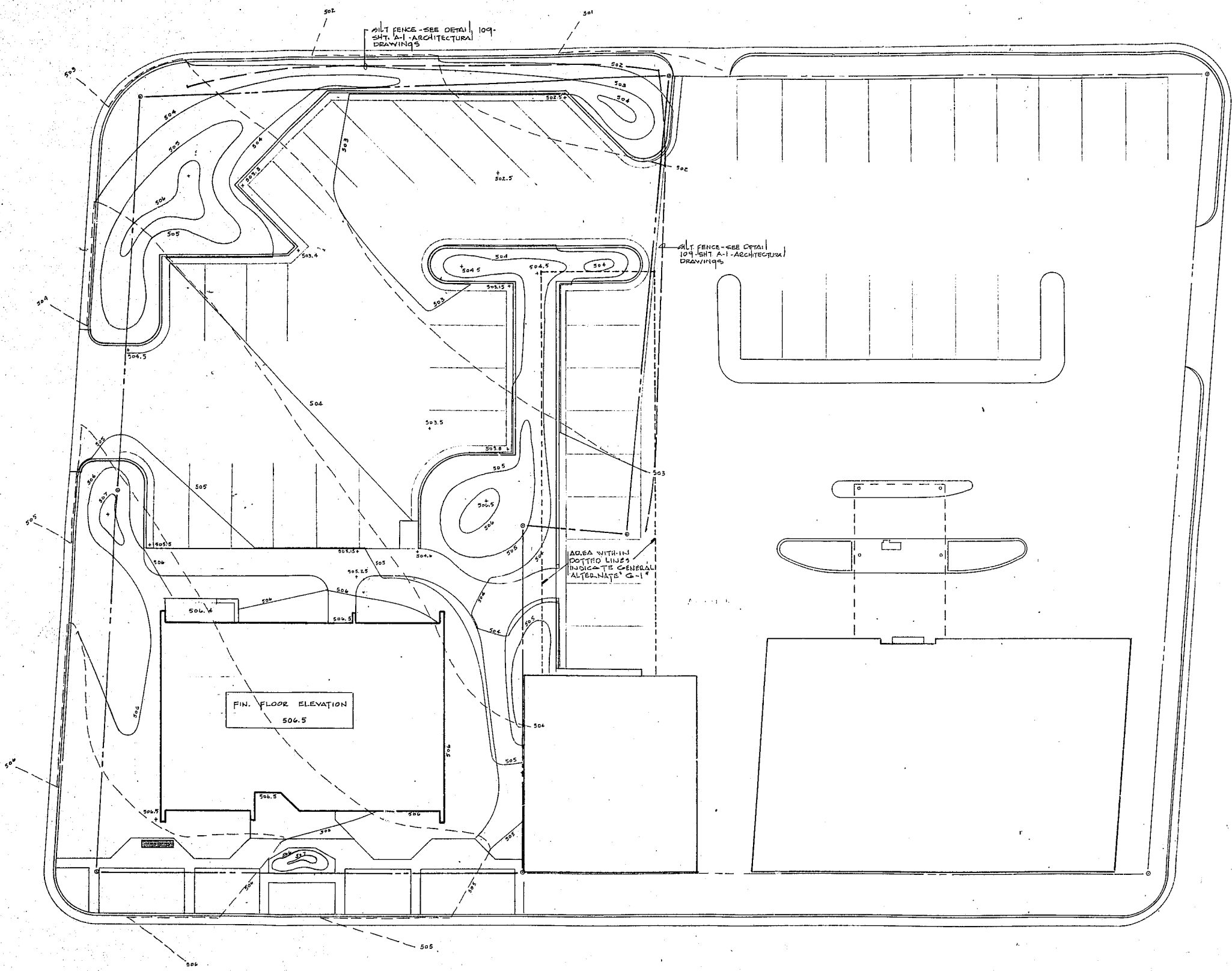
GRADING PLAN SCALE: 1" = 10'-0"
