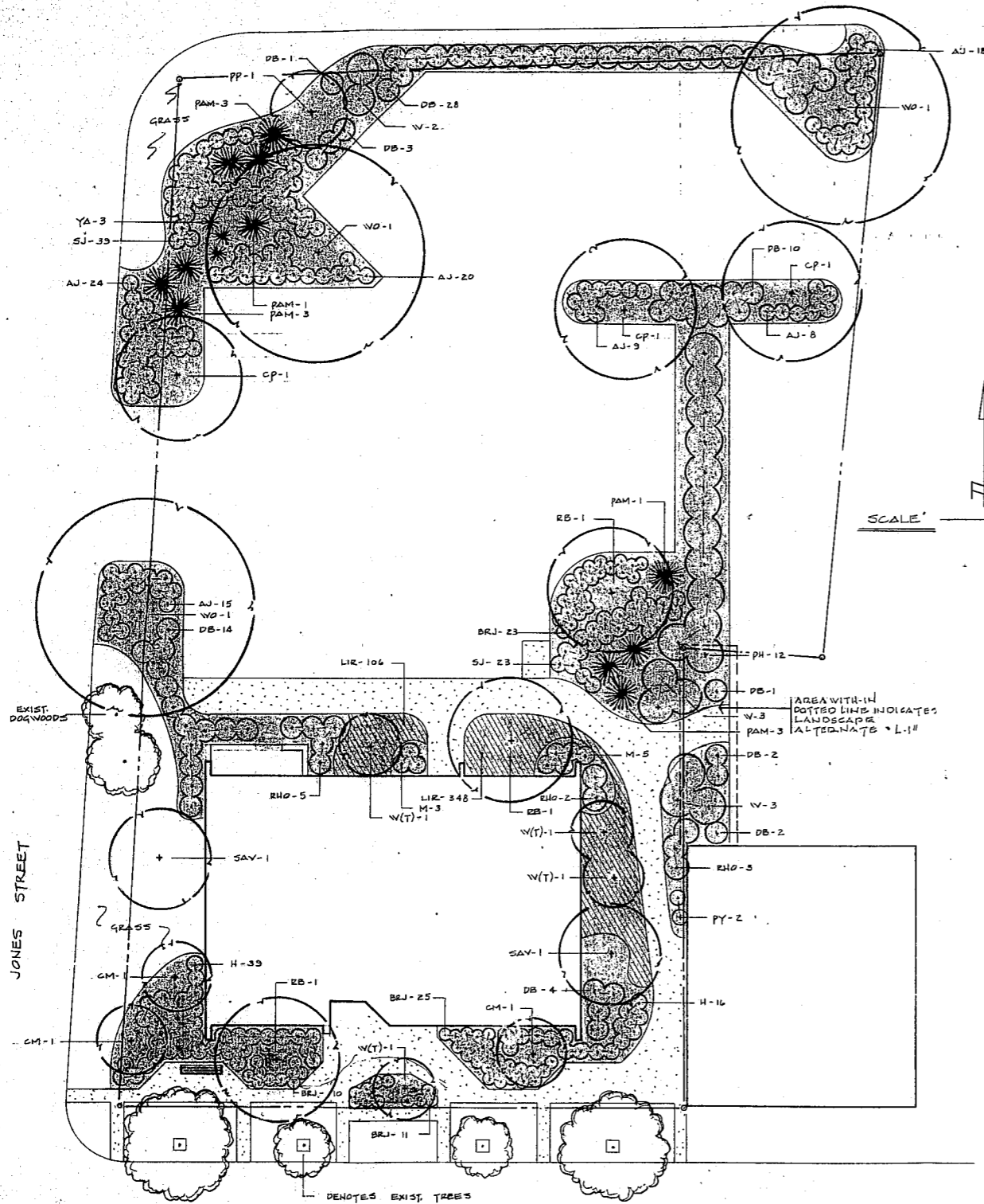
WEST CHATHAM STREET LANDSCAPE PLAN SCALE - 1" = 10'
