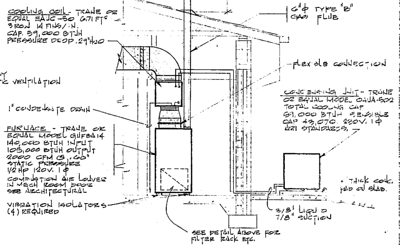
SECTION THRU MECHANICAL ROOM SCALE 3/8" = 1'-0"
