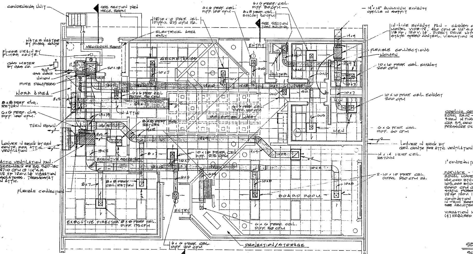
HEATING & AIR CONDITIONING FLOOR PLAN SCALE 1/4" = 1'-0"
