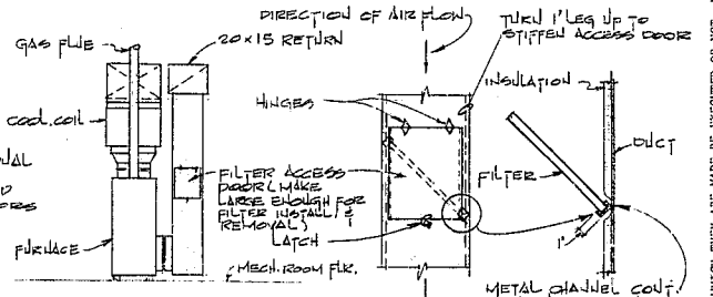
DETAIL OF FILTER RACK SCALE 1/2" = 1'-0"
