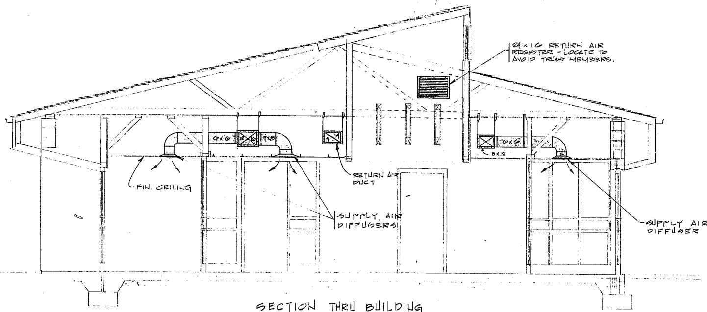
SECTION THRU BUILDING SCALE 3/8" = 1'-0"
