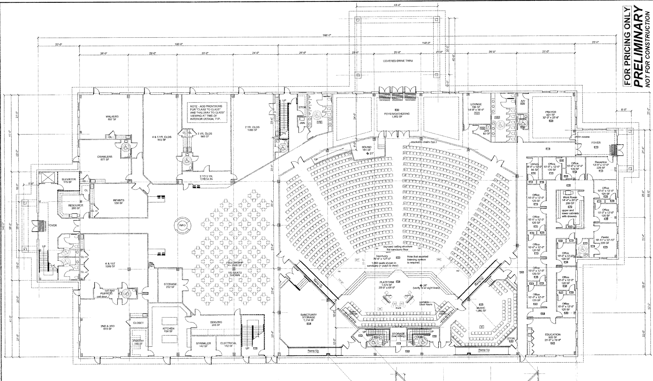
1 FIRST FLOOR PLAN 3/32" = 1'-0"
