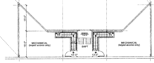
2 MEZZANINE PLAN 3/32" = 1'-0"
