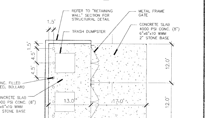
8 DUMPSTER ENCLOSURE LAYOUT DETAIL NTS
