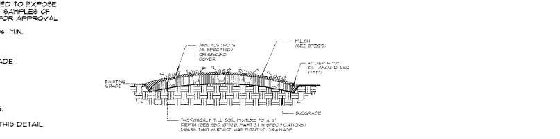
12 GROUND COVER/ANNUALS PLANTING DETAIL NOT TO SCALE
