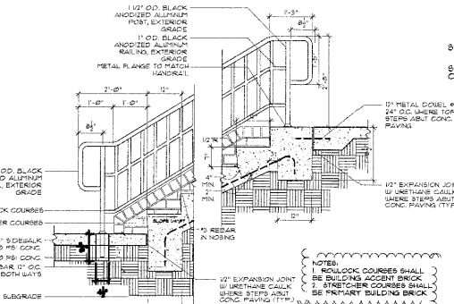
3 STEPS WITH CHEEKWALL AND RAIL NTS
