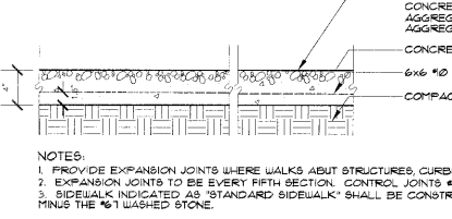
11 TYPICAL SIDEWALK DETAIL NTS
