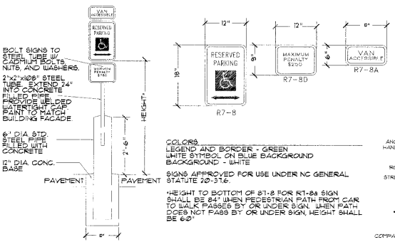
2 HDGP SIGN DETAIL NTS
