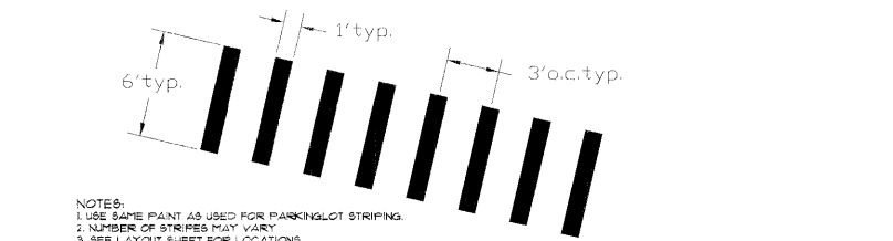
10 TYPICAL CROSSWALK PAINTSTRIP LAYOUT DETAIL NTS
