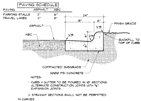
1 SECTION THRU CURB AND GUTTER / PAVING and PAVING SCHEDULE NTS
