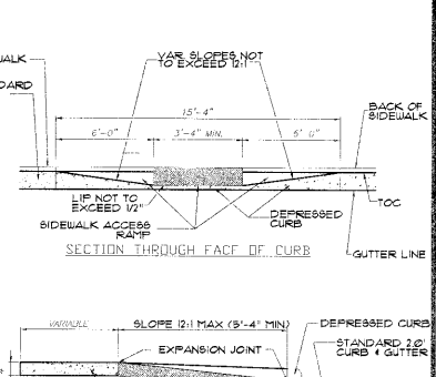
4 TYPICAL HDGP RAMP NTS
