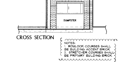
9 DUMPSTER ENCLOSURE DETAILS NTS
