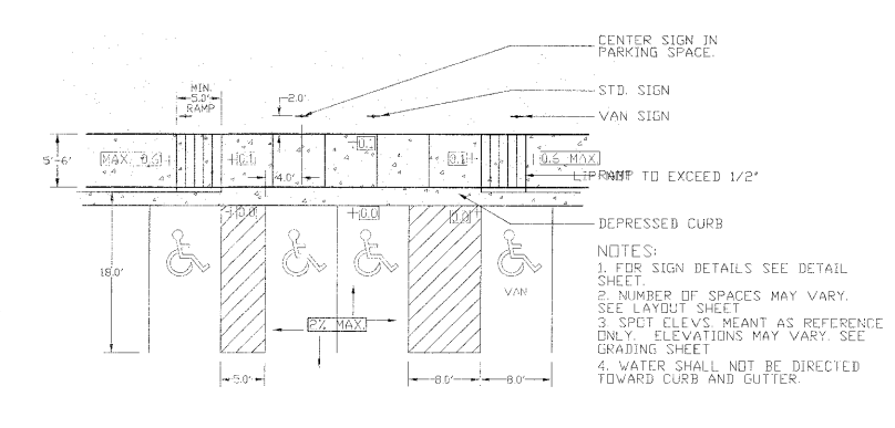
7 TYPICAL HDGP PARKING SPACE LAYOUT NTS
