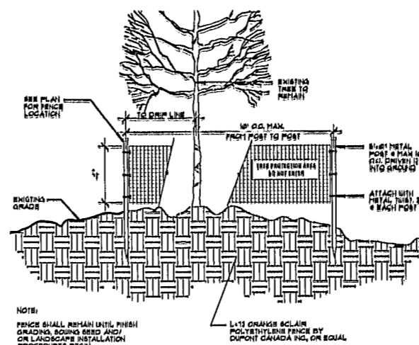
TREE PROTECTION FENCE
