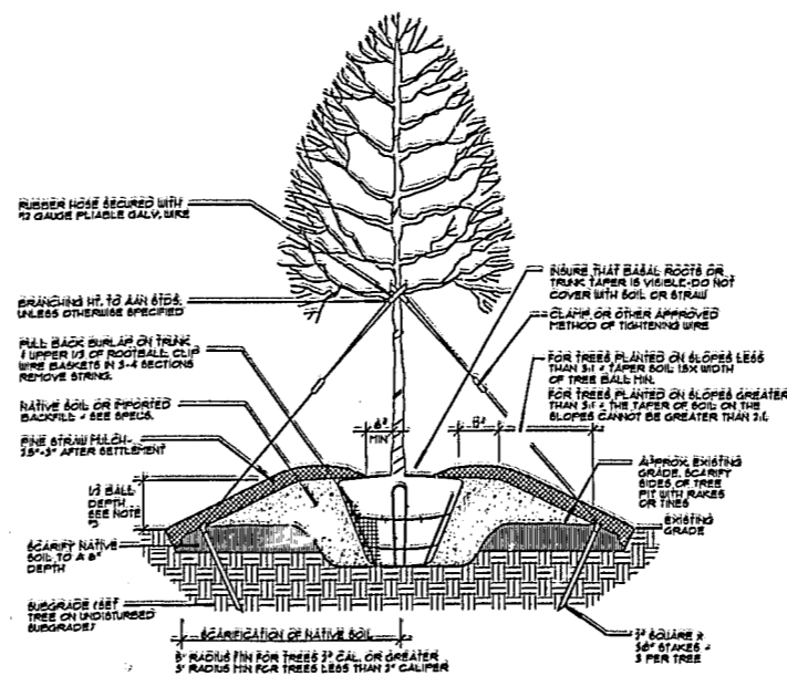
TREE PLANTING DETAILS
