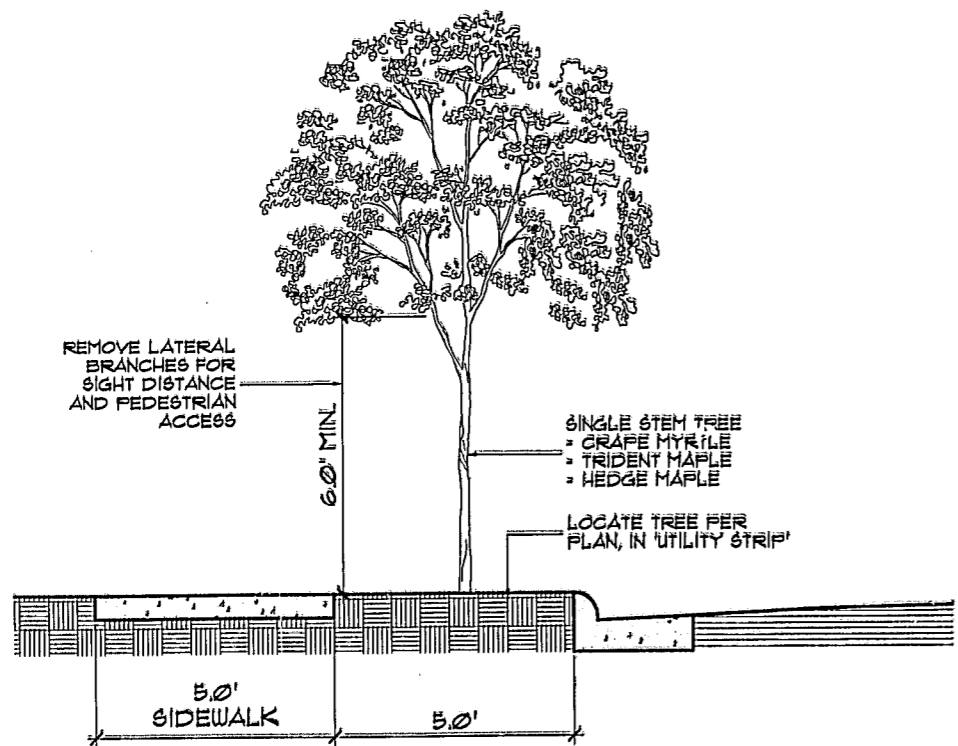
SMALL SCALE STREET TREE
