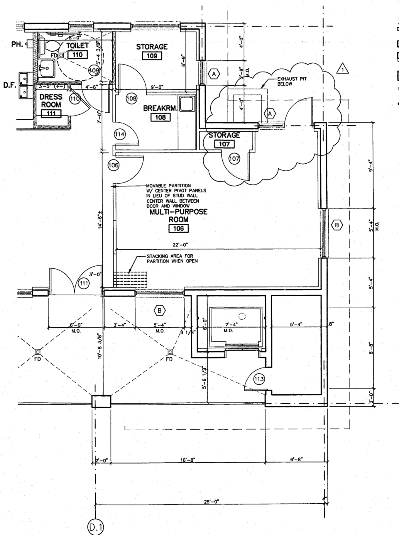
1 FIRST FLOOR PLAN ALTERNATE SCALE: 1/4" = 1'-0"
