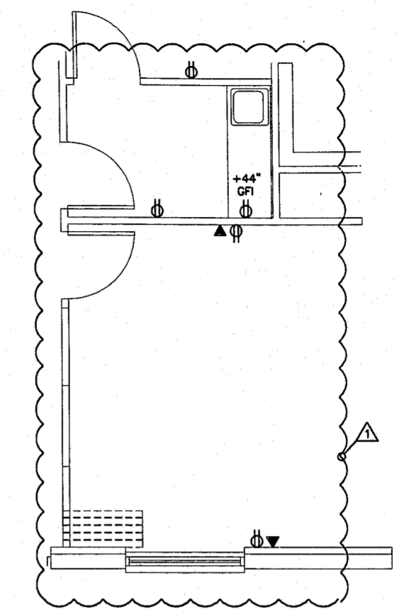
2 PARTIAL FLOORPLAN - ALTERNATE POWER E2.01/SCALE: 1/4" = 1' - 0"
