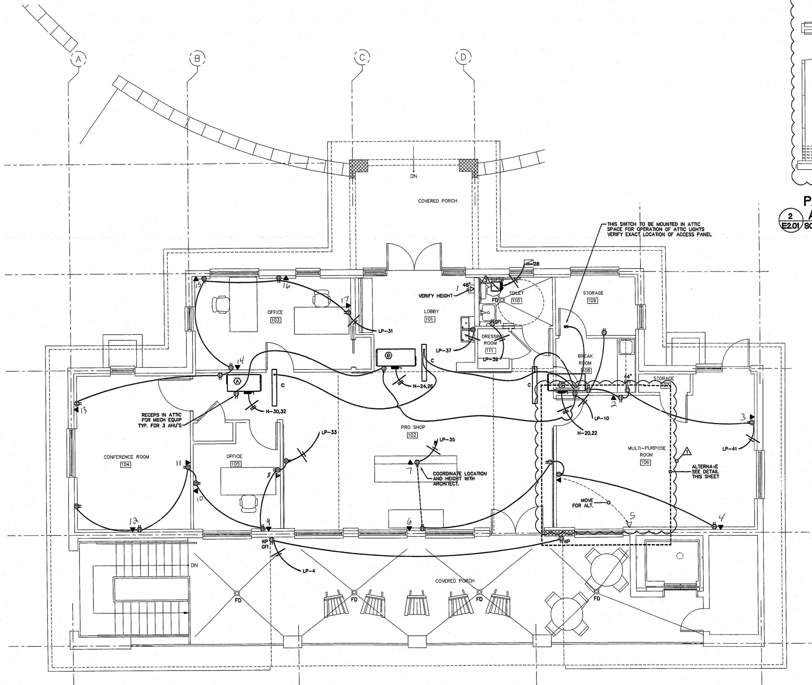
1 FIRST FLOOR PLAN - POWER E2.01/SCALE: 1/4" = 1' - 0"
