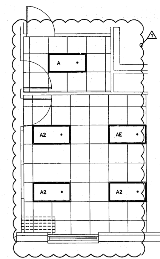
2 PARTIAL FLOORPLAN - ALTERNATE LIGHTING E2.01 SCALE: 1/4" = 1' - 0"
