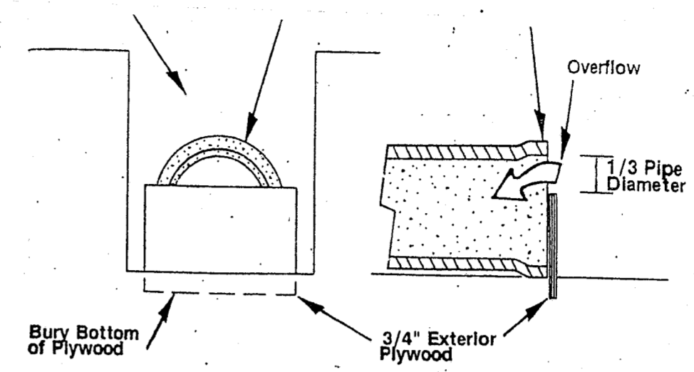
Figure 1: Illustration of Plywood Inlet Protection for Storm Drain Under Construction.
