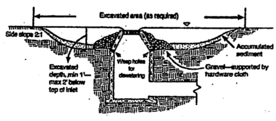
Figure 6.50a: Cross section of excavated drop inlet protection.
