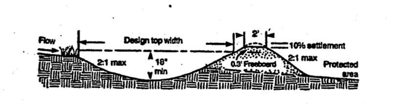
Figure 6.20b: Temporary diversion cross section.
