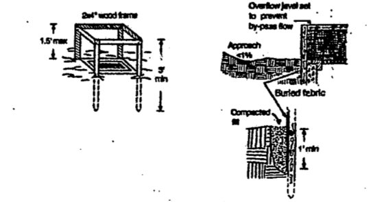
Figure 6.51c: Recommended installation of fabric with supporting frame around storm inlet.
