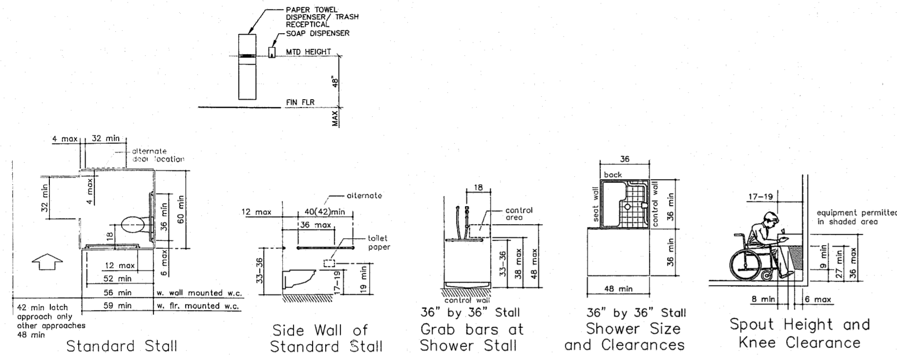
12 ACCESSIBILITY GUIDELINES NO SCALE
