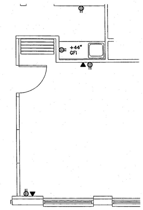
2 PARTIAL FLOORPLAN - ALTERNATE POWER E2.01 SCALE: 1/4" = 1' - 0"
