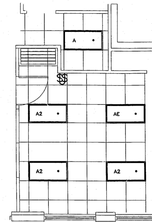
2 PARTIAL FLOORPLAN - ALTERNATE LIGHTING E2.01 SCALE: 1/4" = 1' - 0"
