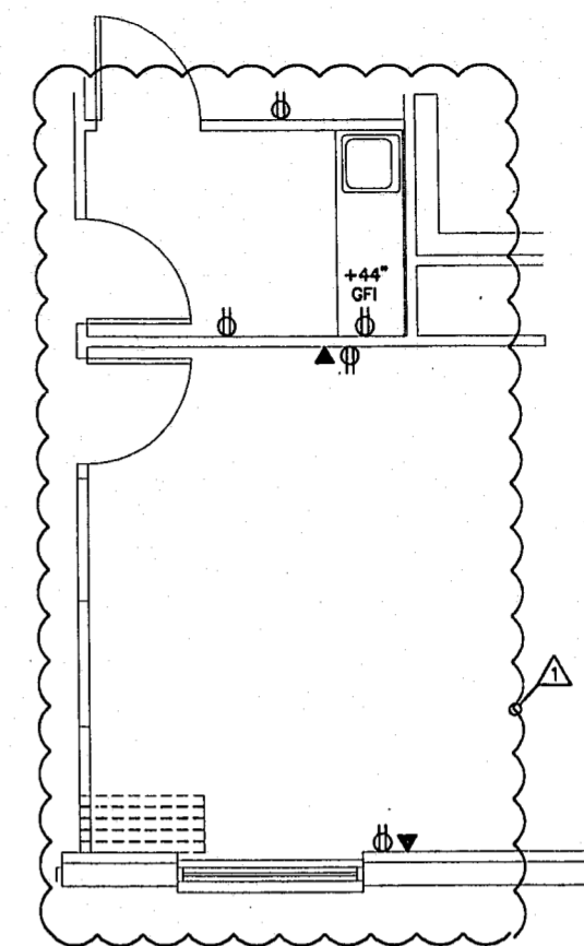
2 PARTIAL FLOORPLAN - ALTERNATE POWER E2.01 SCALE: 1/4" = 1' - 0"
