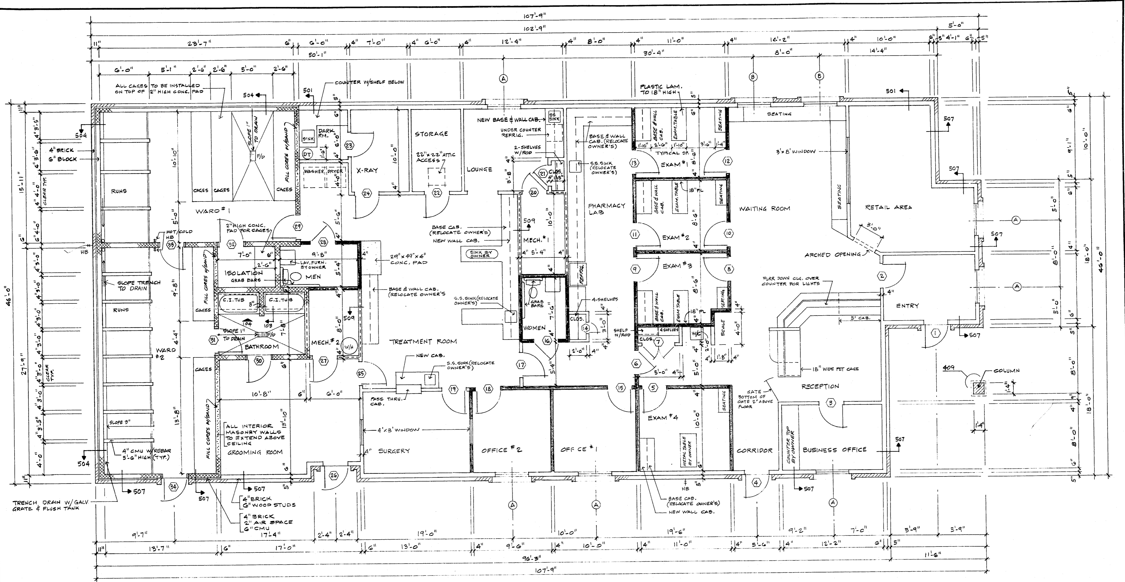
201 FLOOR PLAN 1/4" = 1'-0"
